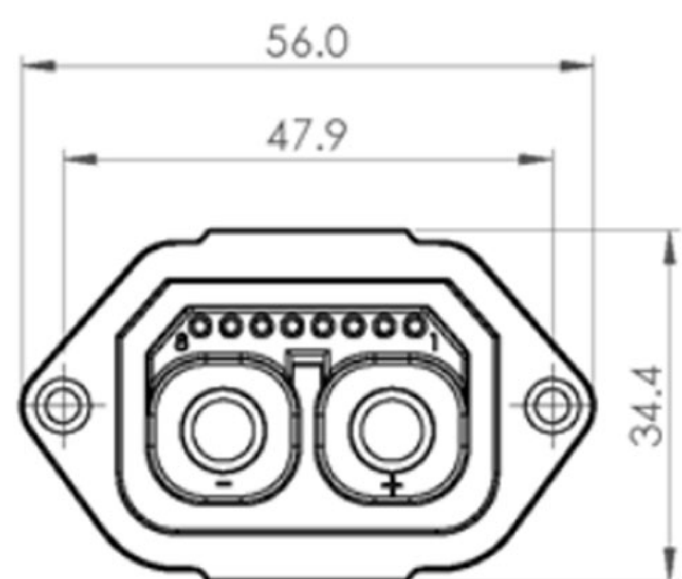
Female Connector
