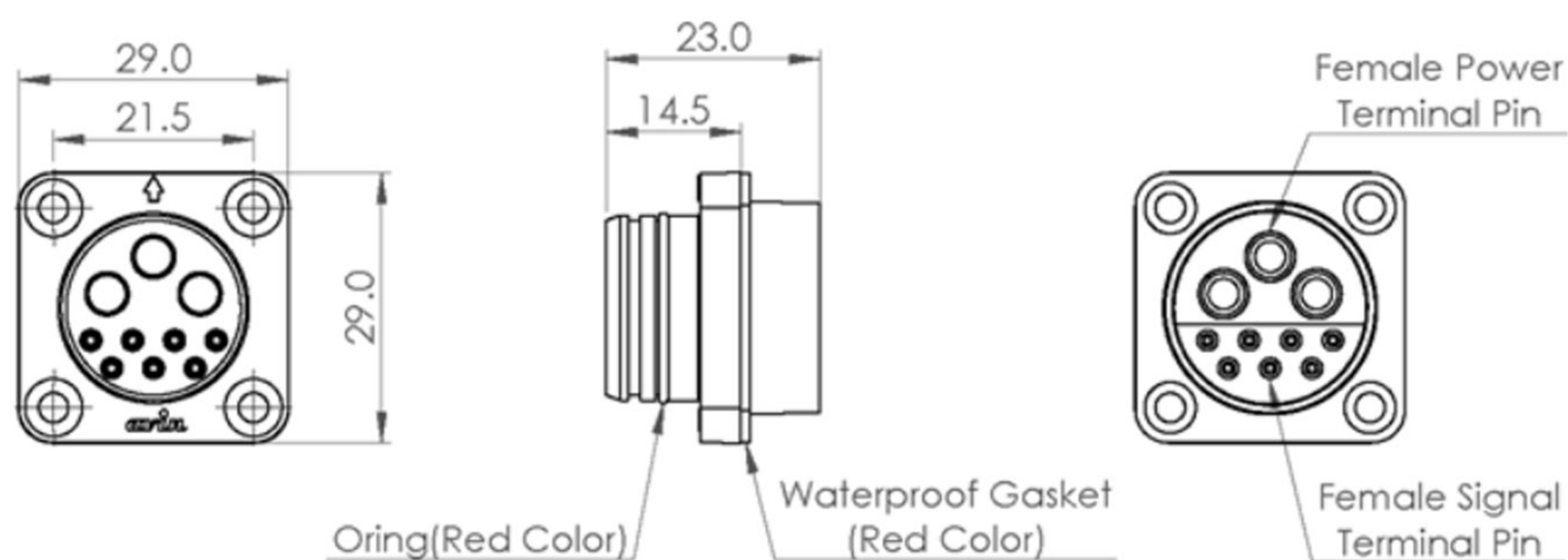
Female Connector
