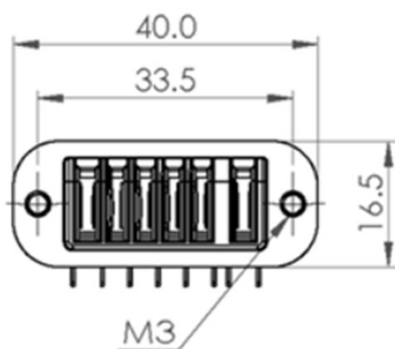
Female Connector
