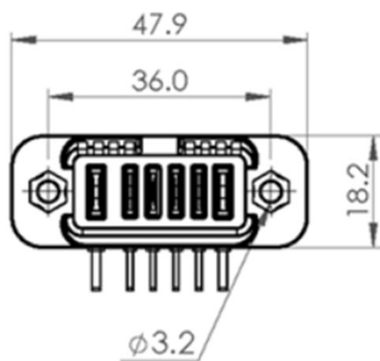
Female Connector
