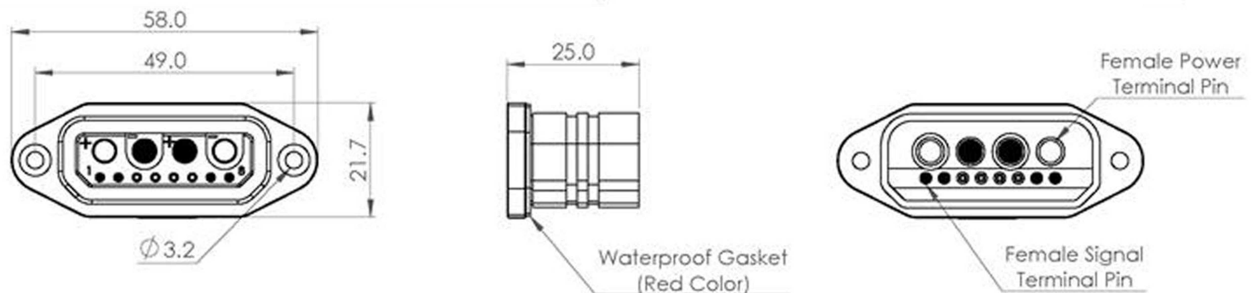
Female Connector
